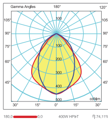
Symmetric Floodlight
