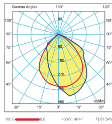
Asymmetric Floodlight
