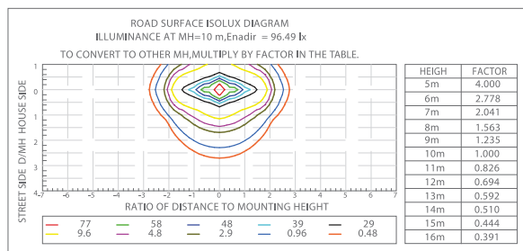
Isolux Diagram*
