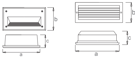
Technical Drawing
